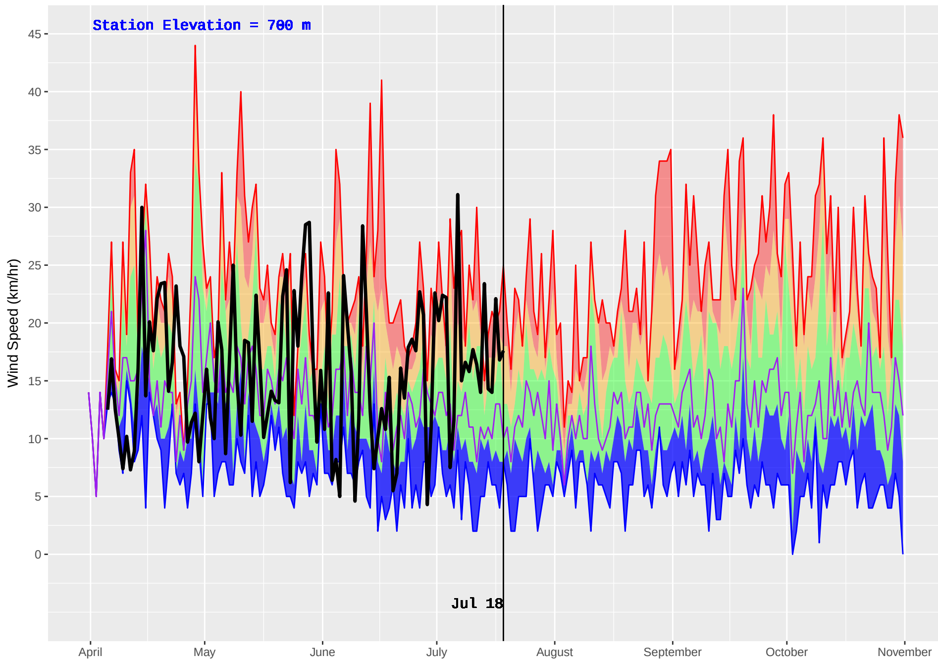
OSBORN (1045) : Historical (2009–2016) and Current (2018) Daily Wind Speed
