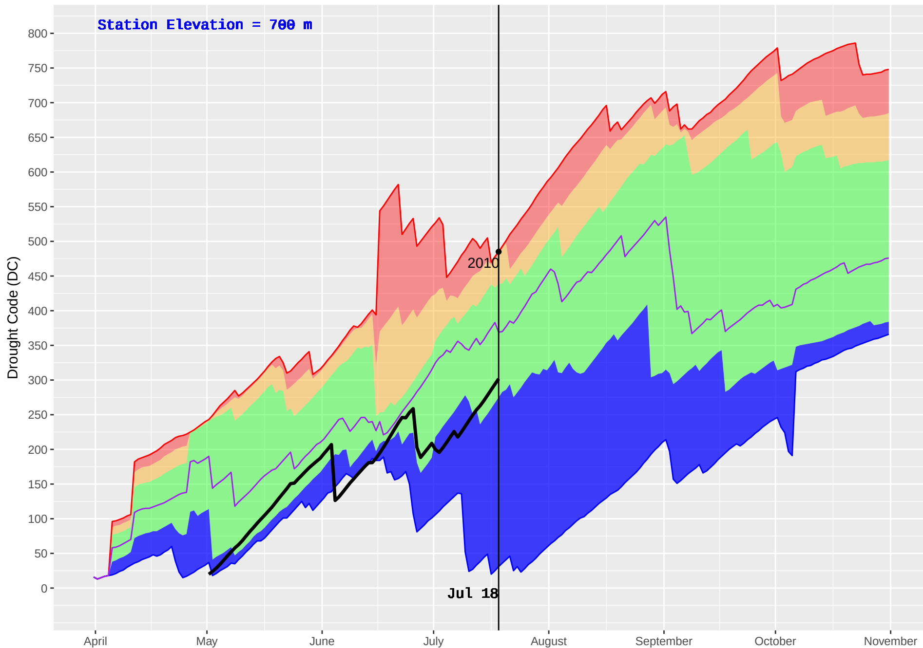
OSBORN (1045) : Historical (2009–2016) and Current (2018) Daily Drought Code (DC)
