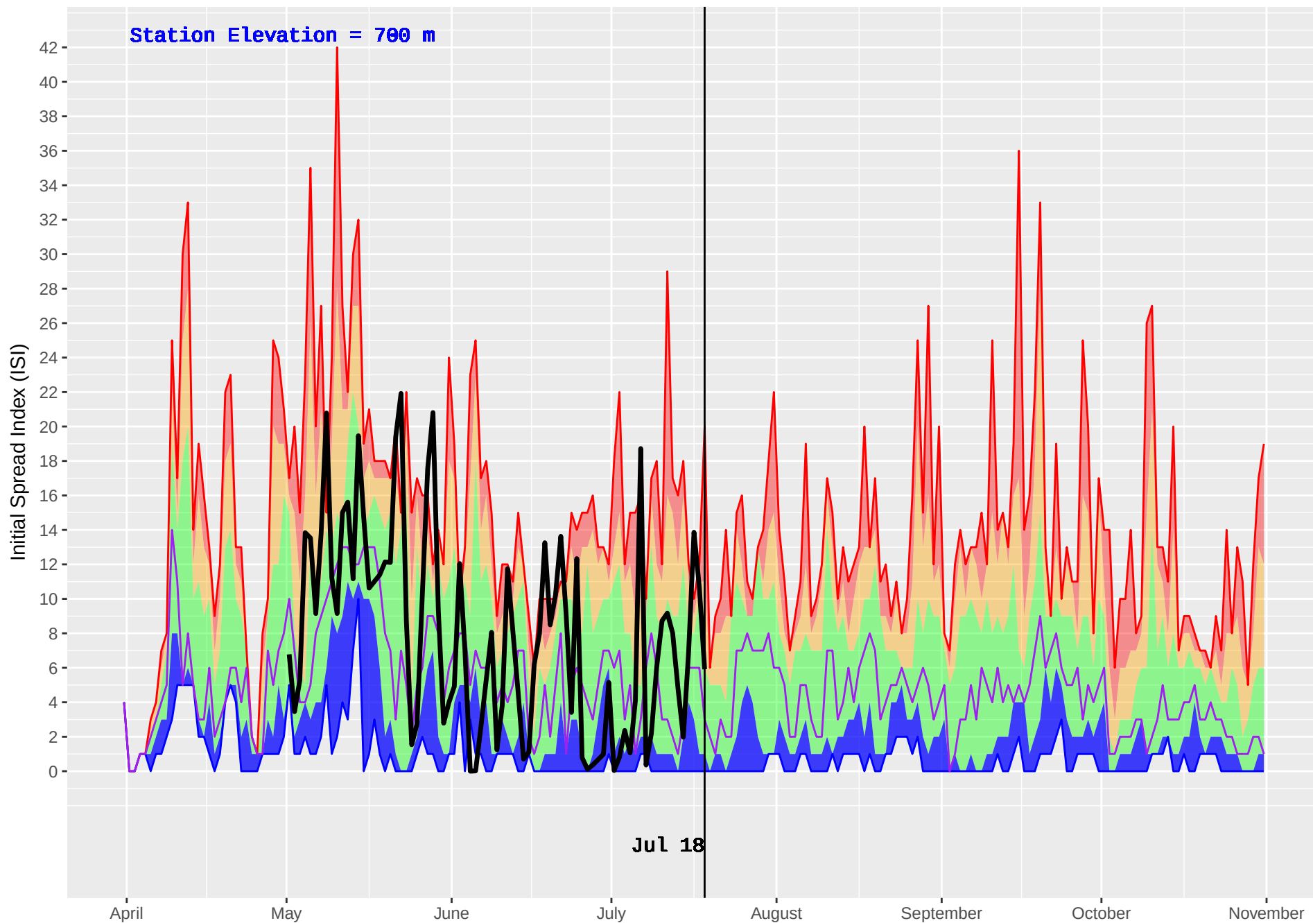
OSBORN (1045) : Historical (2009–2016) and Current (2018) Daily Initial Spread Index (ISI)
